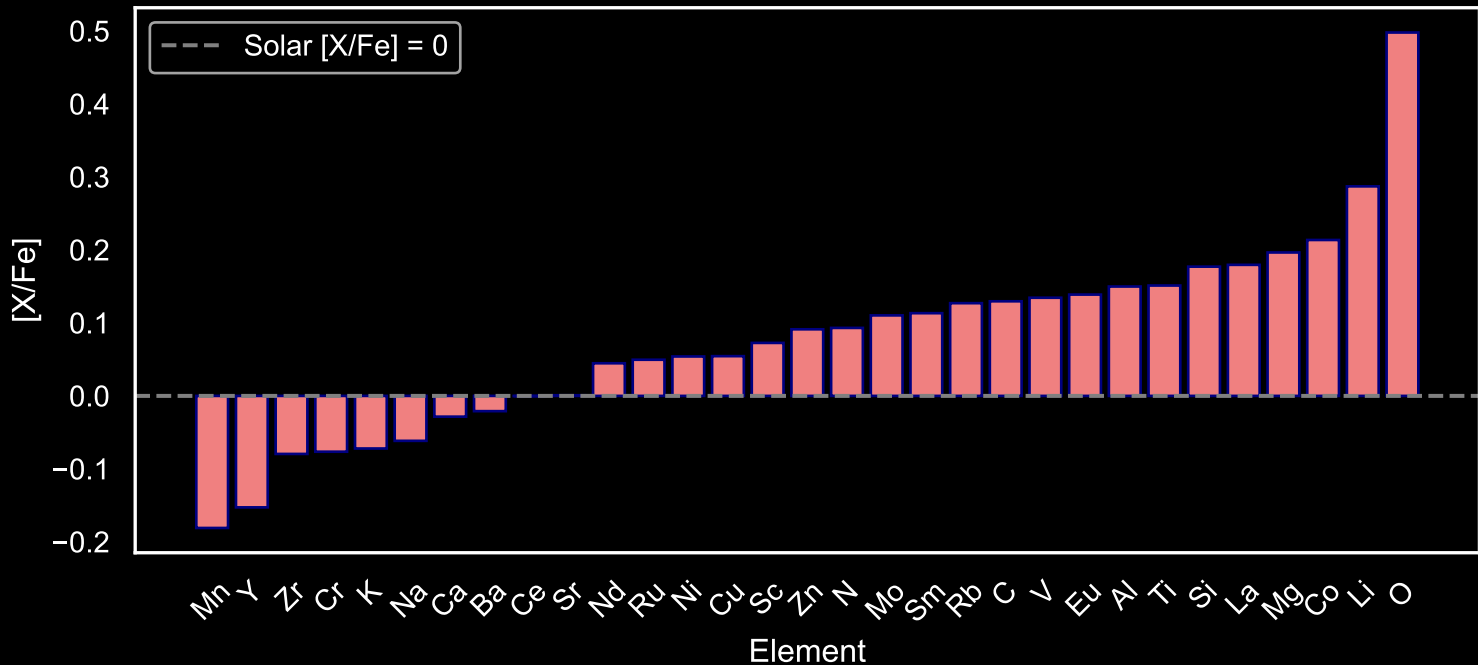
Abundance Pattern for GALAH Red Giants: Star Field [29] (N=50)
