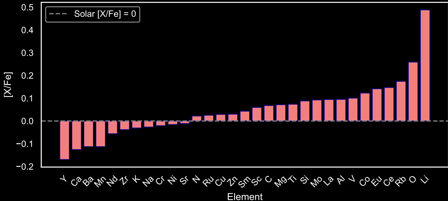
Abundance Pattern for GALAH Star Field [29] (N=203)
