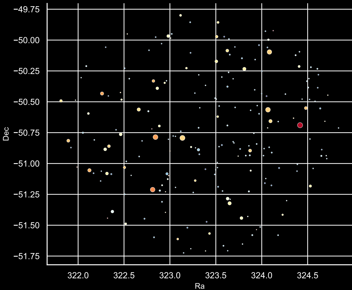
Field [29] Ra [323.44] Dec [-50.74] Stars: 203
