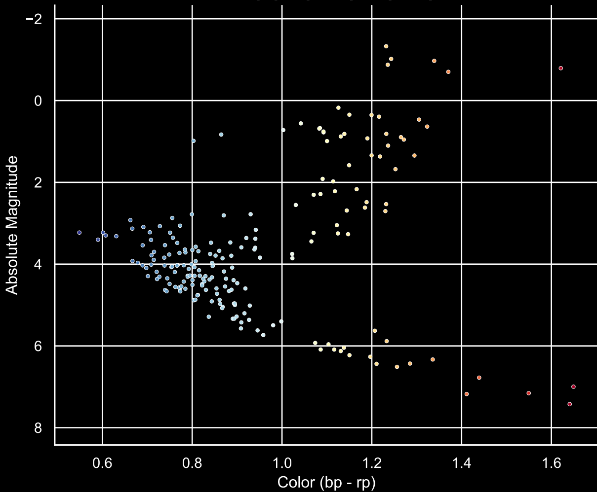
GALAH Hertzprung-Russel Diagram Field [29] Ra [323.44] Dec [-50.74]
