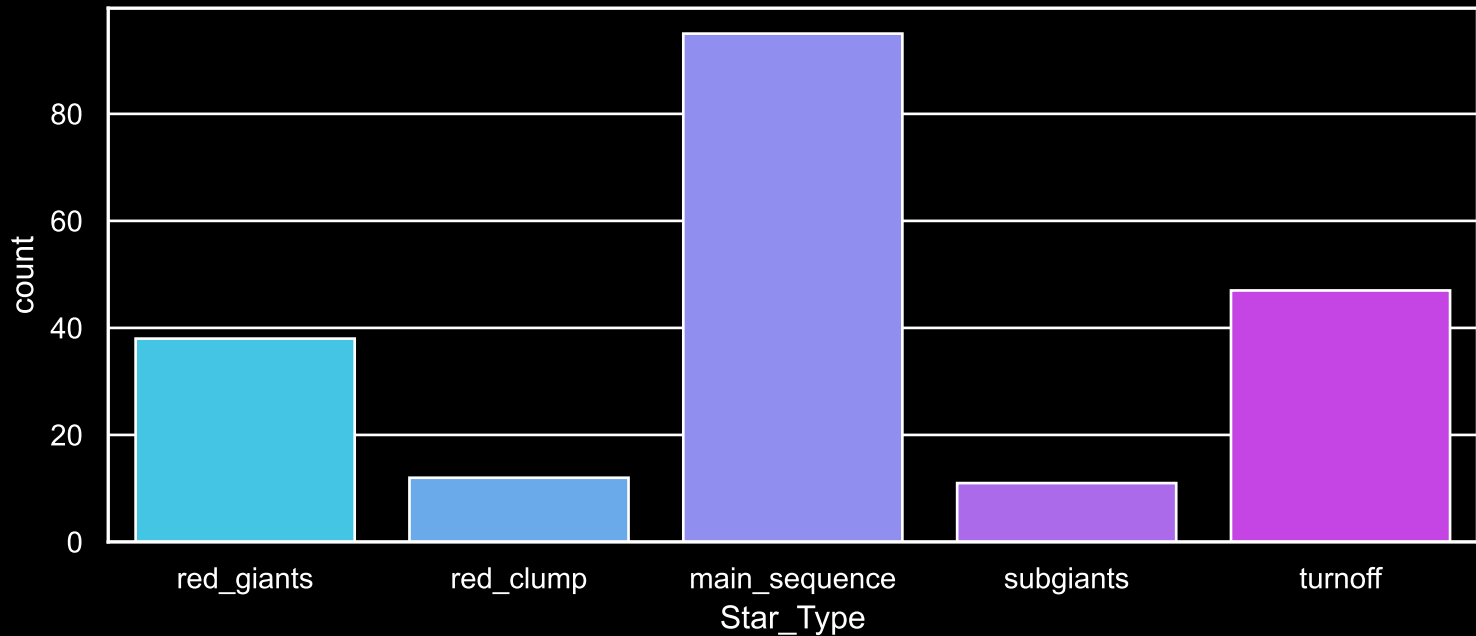
Field [29] Count plot of Star Type
