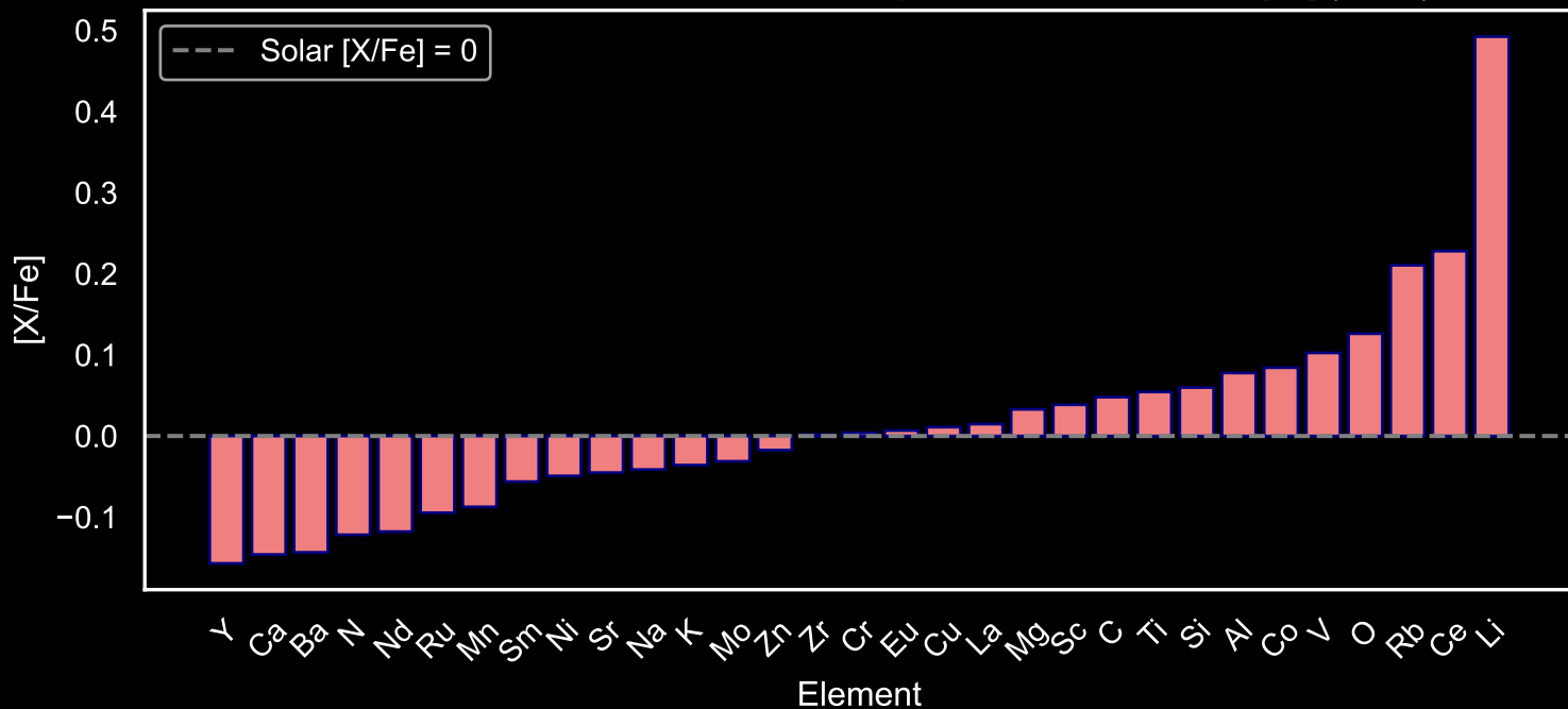
Abundance Pattern for GALAH Main Sequence Stars: Star Field [29] (N=95)
